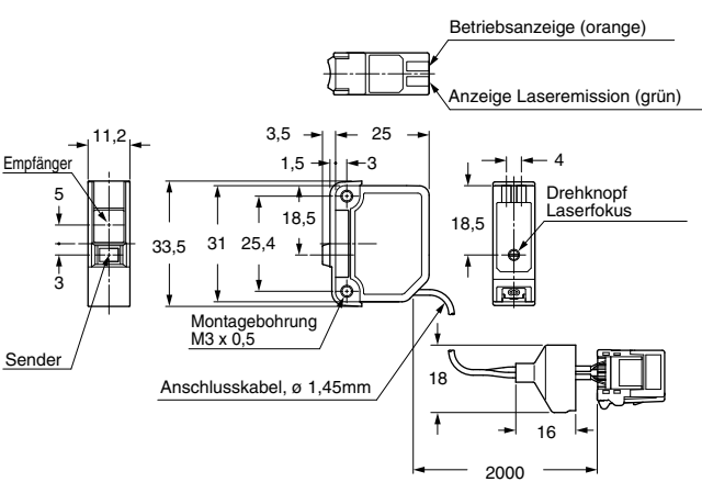
LS-H22 Sensorkopf
