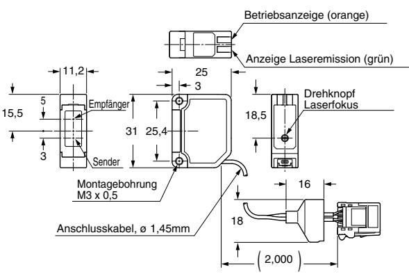
LS-H21 Sensorkopf
