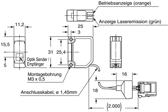
LS-H91, LS-H92 Sensorkopf
