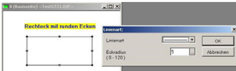
Dialogfeld "Linienart"
